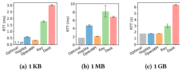
Figure 6: Round trip latency for point-to-point data communication on Hoplite, OpenMPI, Ray, and Dask. We also include the theoretical optimal RTT (i.e. total bytes transferred divided by the bandwidth).
